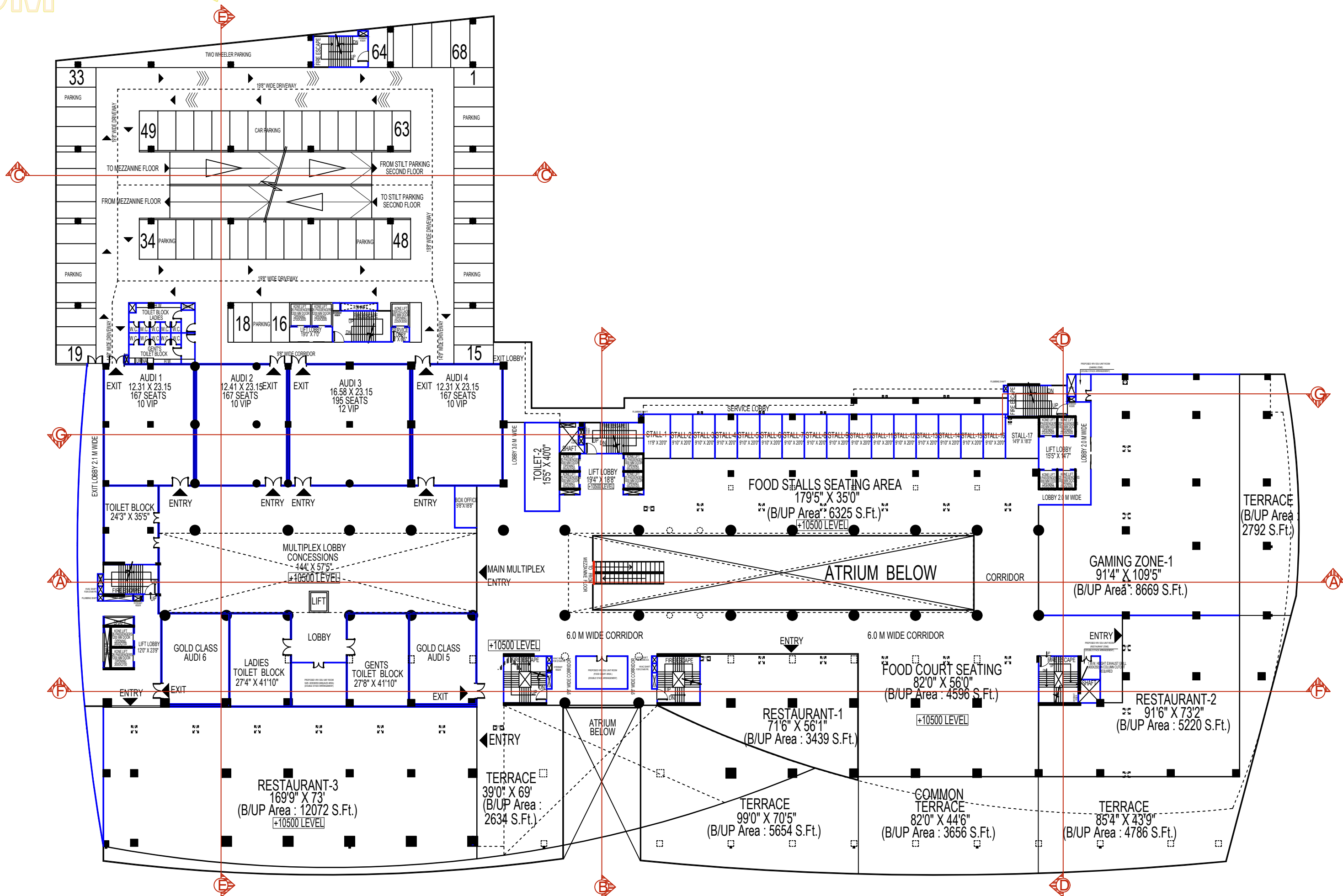
FIRST FLOOR PLAN MULTIPLEX & FOOD COURT LEVEL
